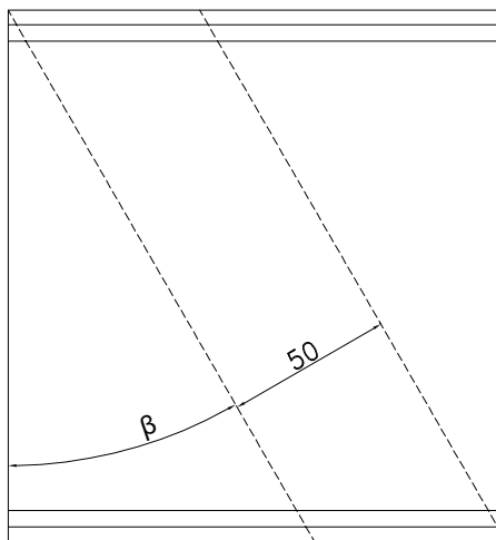
Primjer pilanja spojnice okomice Example of sawing of the mullion connection
