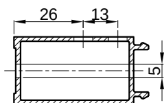
Nosač F-1129 gore Support profile F-1129 up
