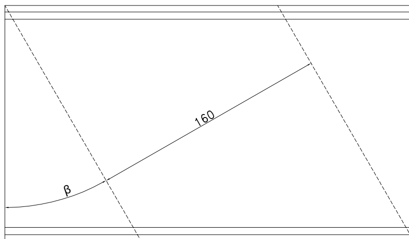
Primjer pilanja spojnice okomice Example of sawing of the mullion connection
