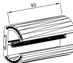
722.002 (za FMV 60/114) (for FMV 60/114)
