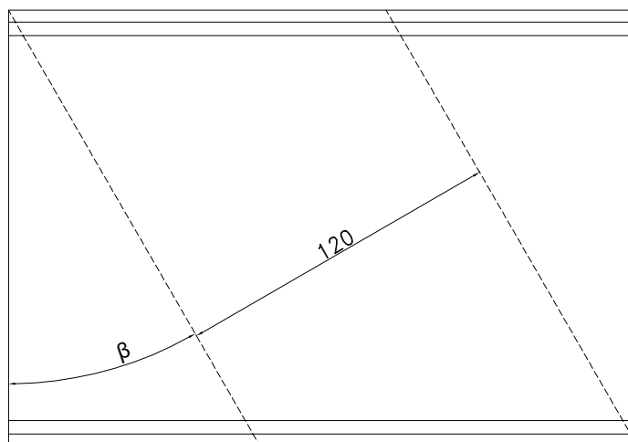
Primjer pilanja spojnice okomice Example of sawing of the mullion connection
