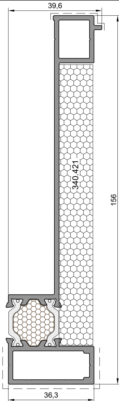
Spojni profil sa fasadom Connection profile for curtain wall
