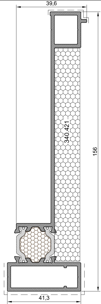
Spojni profil sa fasadom Connection profile for curtain wall
