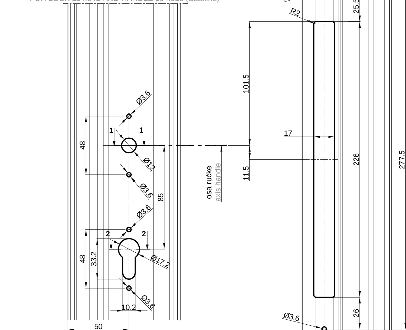
PRESJEK 1-1 CROSS SECTION 1-1
