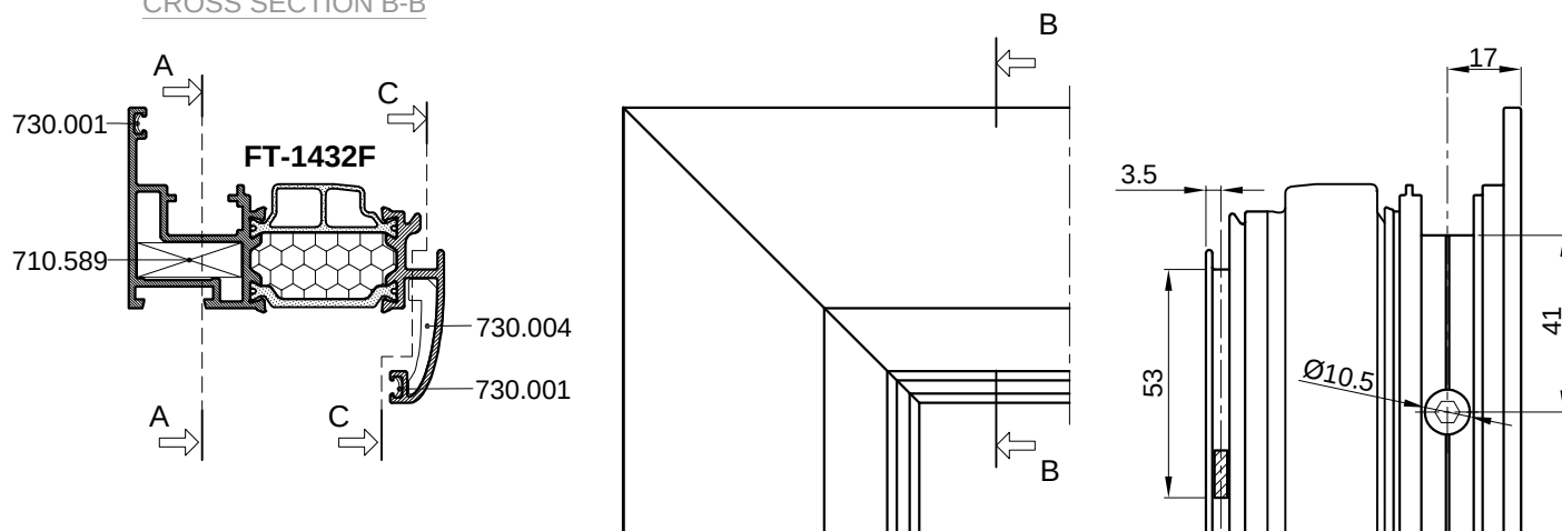
CROSS SECTION B-B
