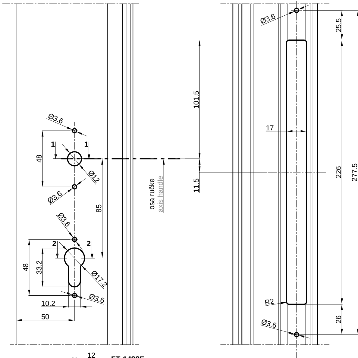
PRESJEK 1-1 CROSS SECTION 1-1
