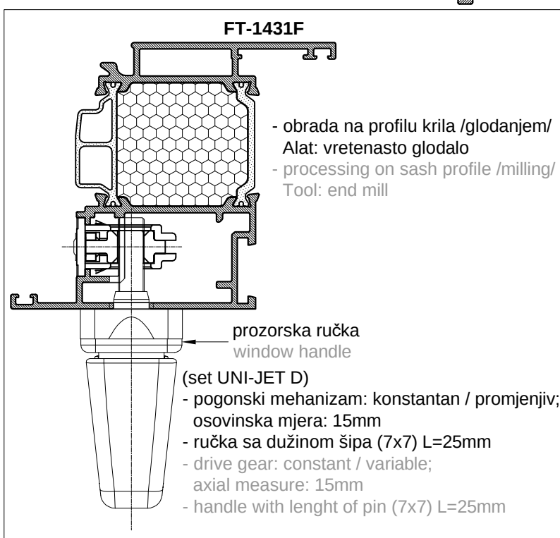
PRESJEK 3-3 CROSS SECTION 3-3
