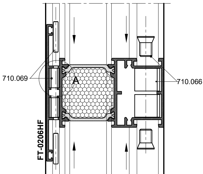
DETAIL A DETAIL A M 5:1
