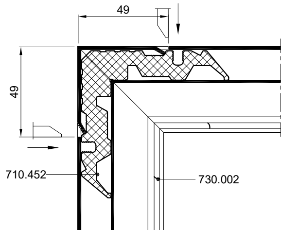
PRESJEK C-C CROSS-SECTION C-C
