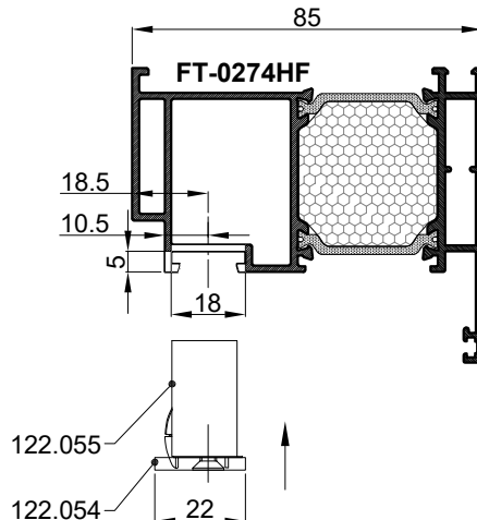
PRESJEK 2-2 CROSS SECTION 2-2
