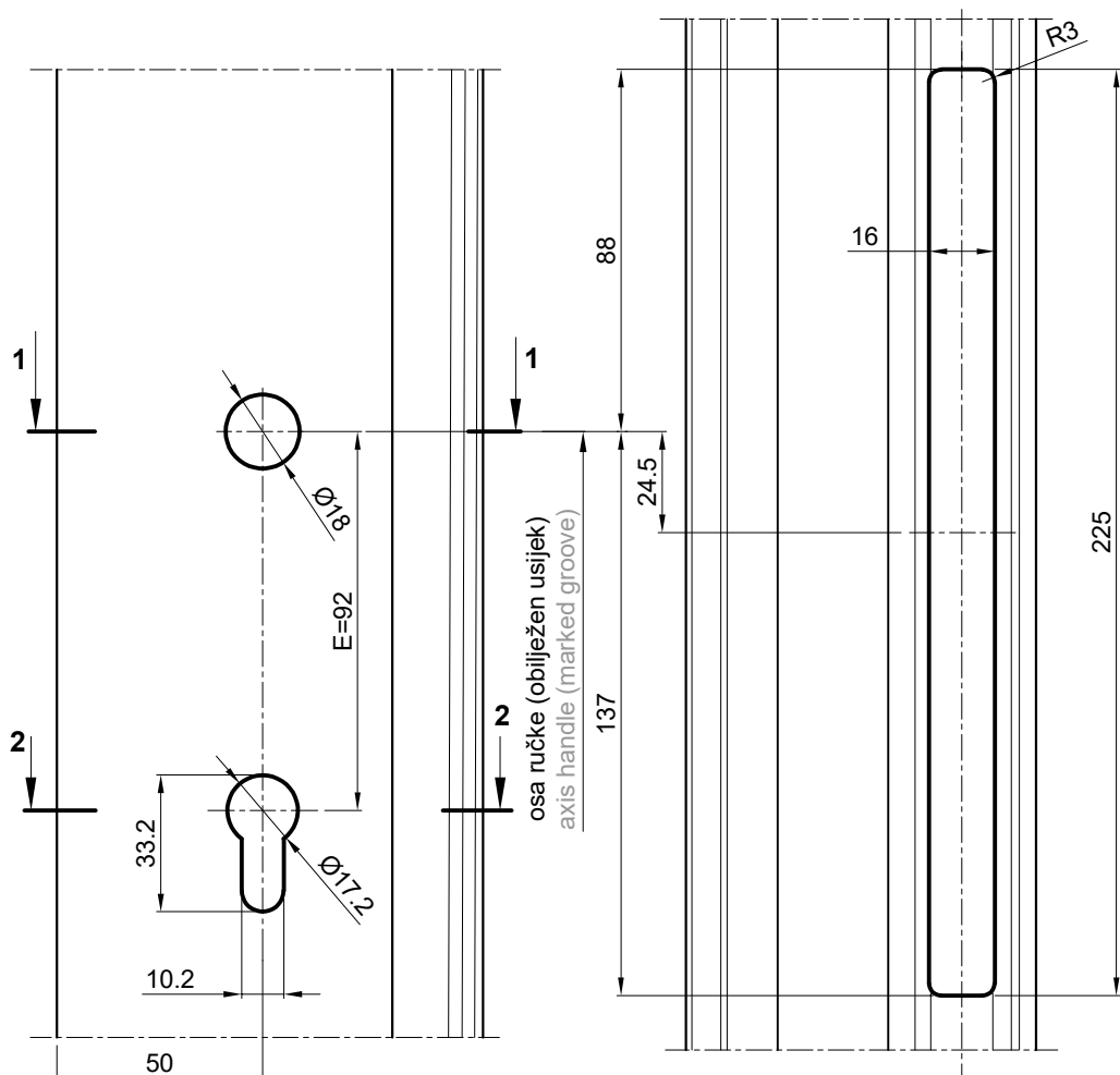
PRESJEK 1-1 CROSS-SECTION 1-1
