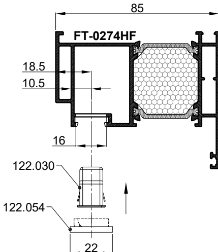
PRESJEK 1-1 CROSS SECTION 1-1
