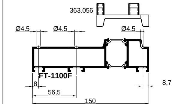
Obrada profila FT-1100F Processing profile FT-1100F
