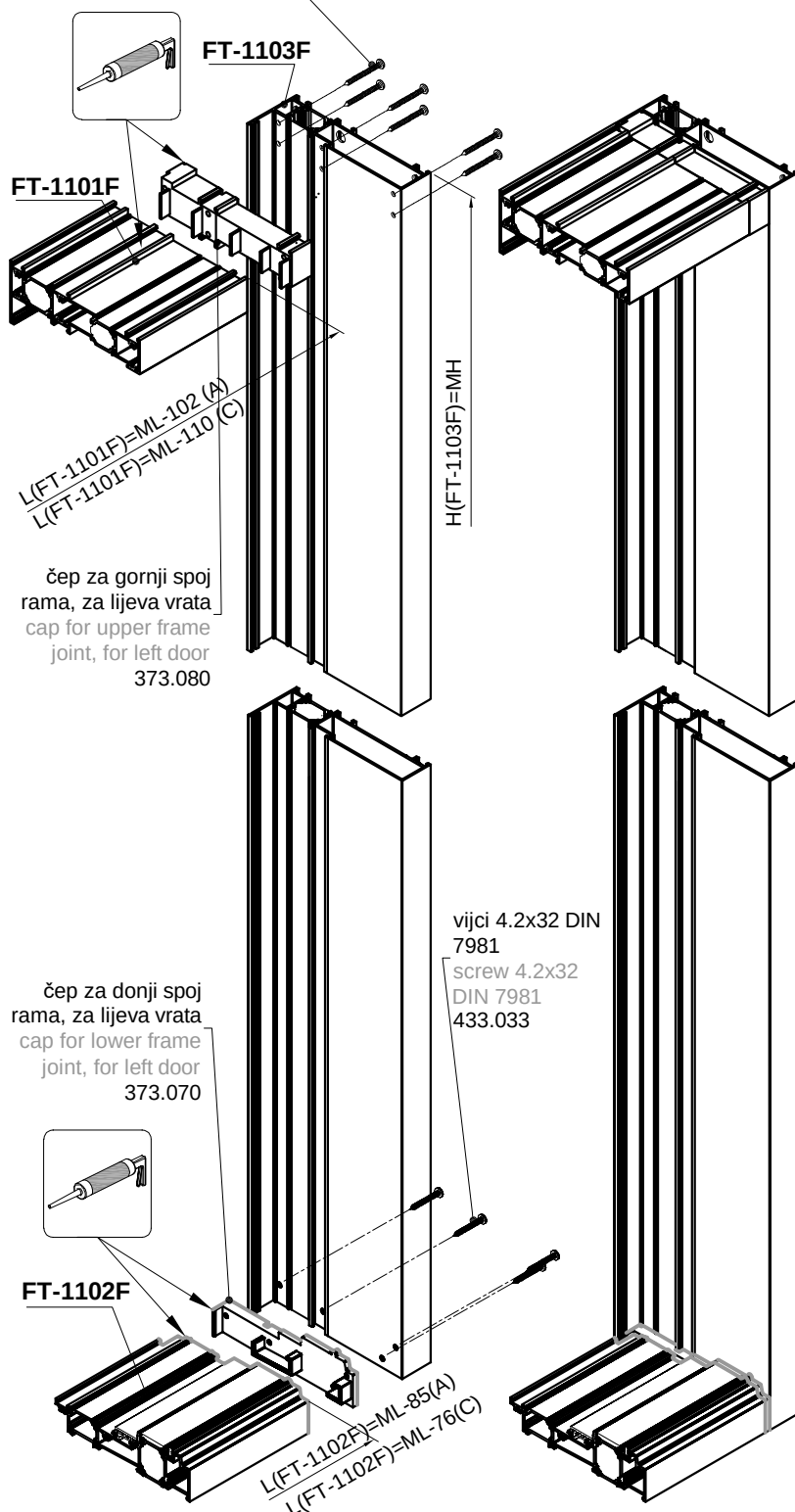
Obrada profila FT-1103F Processing profile FT-1103F
