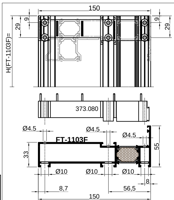
Obrada profila FT-1103F Processing profile FT-1103F
