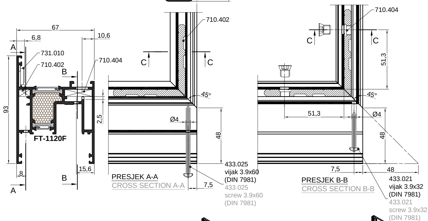
SPAJANJE PROFILA FT-1120F SA PROFILIMA KRILA FT-1121 I FT-1122 KUTNICIMA PROFILES CONNECTION FT-1120F WITH SASH PROFILES FT-1121 AND FT-1122 WITH CORNER BRACKETS
