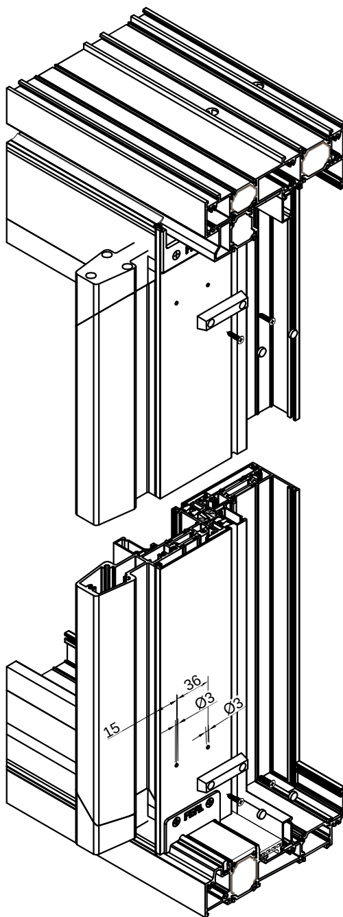
Obrada profila F-1538 Processing profile F-1538
