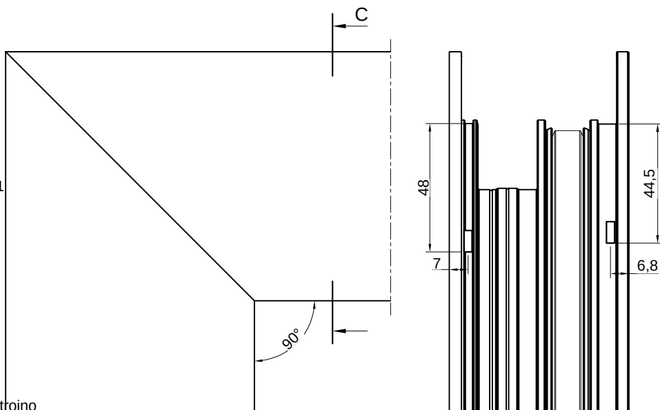
SPAJANJE PROFILA FT-1120F KUTNICIMA CONNECTION PROFILE FT-1120F WITH CORNER BRACKETS
