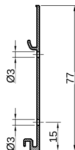
Obrada profila F-1538 Processing profile F-1538
