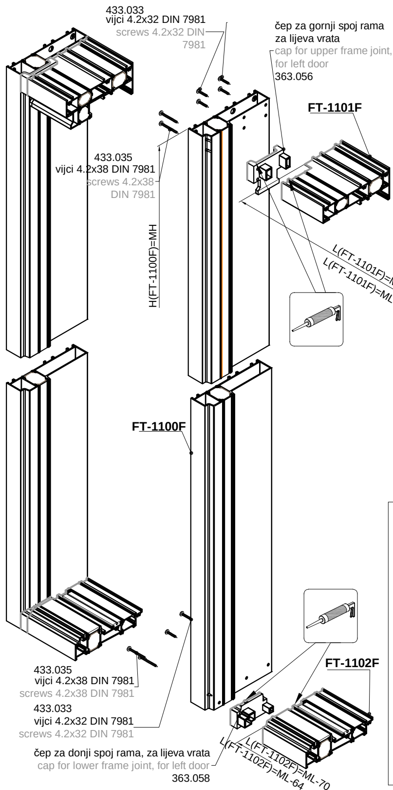
Obrada profila FT-1100F Processing profile FT-1100F
